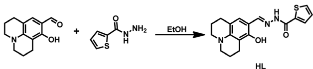
Fig. 1 Synthetic route of HL.
