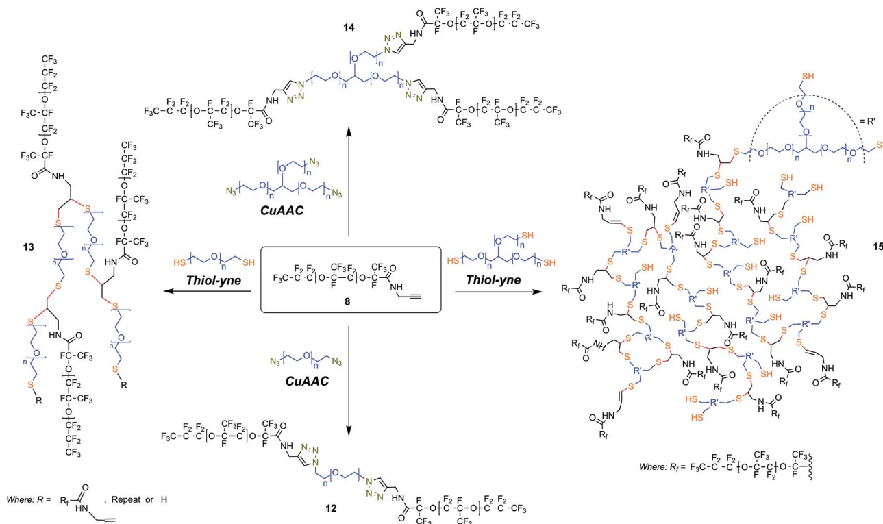
Fig. 3 Surfactant synthesis and resulting structure diversity highlighting the central role played by the intermediate Krytox propargyl amine (8) that can be combined with either a homo-bifunctional PEG or a 3-arm homo-functional glycerol ethoxylate by CuAAC or thiol-yne reactions. Those reactions permit the generation of PFPE-PEG surfactants with a variety of structures. CuAAC (12): 10 mol% Cu(OAc) 2 , 20 mol% sodium ascorbate, 16 mol% neocuproine; 1 : 1 HFE 7100 : 1 : 1 MeOH/H 2 O, 60 °C, 48 h, thiol-yne (13): 0.2 equiv. DMPA, UV 365 nm; 2 : 1 HFE 7100 : MeOH, RT, 48 h, CuAAC (14): 15 mol% Cu(OAc) 2 , 35 mol% sodium ascorbate, 30 mol% TBTA; 1 : 1 HFE 7500 : 2 : 1 MeCN/H 2 O, 80 °C, 48 h, thiol-yne (15): 0.2 equiv. DMPA, UV 365 nm; 2 : 1 HFE 7100 : MeOH, RT, 48 h.
