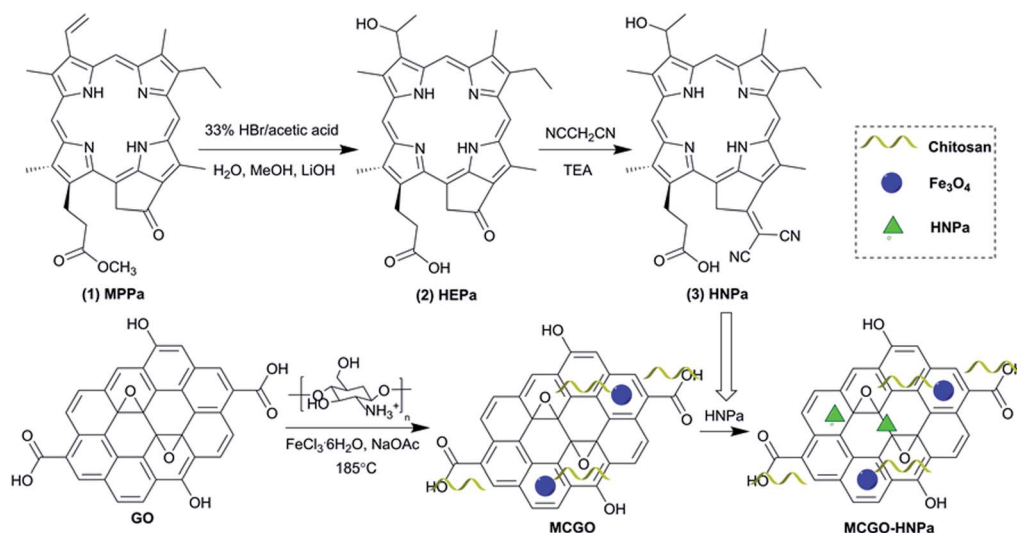
Scheme 1 Schematic of the preparation of MCGO–HNPa composite.
