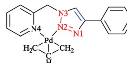
Scheme 20 Structure of the [Pd(\eta^3-C_3H_5)(2-((4-phenyl-1H-1,2,3-triazol-1-yl)methyl)-pyridine)]^+ complex.
