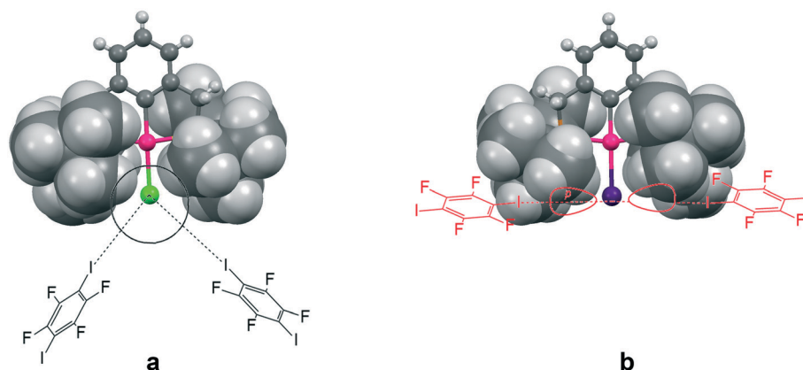
Fig. 10 The tert -butyl fragment of a (2,6-bis[(di- tert -butylphosphino)methyl]phenyl)PdX (ref. 6) (X = Cl (a) and I (b)) complex is shown as a space filling model to demonstrate the shielding of the 5p equatorial "belt" of the iodide ligand (b), as compared to the spherical chloride "anion" (a), escaping the shield.
