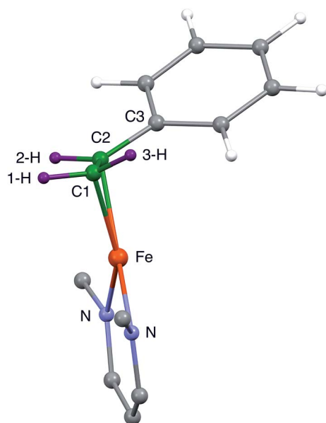
Fig. 3 Side view of the core of the DFT model of 1, showing that the phenyl group is displaced away from the di-tert-butylaminate supporting ligand. This tilts the plane of the alkene and also places C2 further than C1 from Fe.
