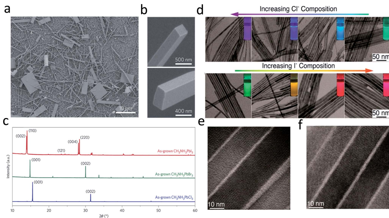
Fig. 4 (a) and (b) SEM images of \text{CH}_3\text{NH}_3\text{PbI}_3 nanostructures. (c) PXR patterns of as-grown \text{CH}_3\text{NH}_3\text{PbX}_3 ( X = \text{I}, \text{Br}, \text{Cl} ) NWs. (d) TEM images of \text{CsPbX}_3 NWs with various degrees of conversion with chloride and iodide anions. The insets show the evolution of emission color (UV excitation, \lambda = 365 nm) upon forming mixed-halide \text{CsPb}(\text{Br}/\text{Cl})_3 and \text{CsPb}(\text{Br}/\text{I})_3 NWs. HRTEM images of (e) Cl- and (f) I-exchange NWs. Reprinted with permission from ref. 15 and 74, copyright 2015, Nature Publishing Group and 2016, American Chemical Society.
