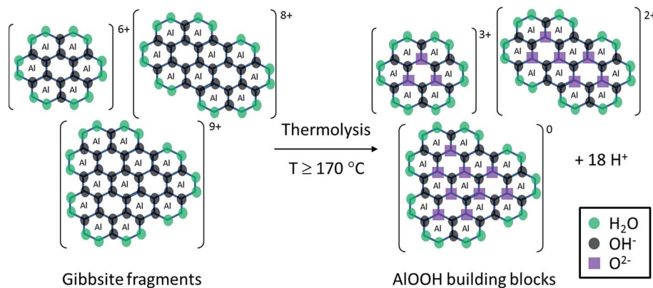
Fig. 2 Representation of the transformation of planar gibbsite fragments to AIOOH building blocks by thermolysis. Each small hexagon represents an octahedral arrangement of atoms around the Al atom. Ligands are colour coded with green, black and purple representing H 2 O, OH - and O 2- respectively.
