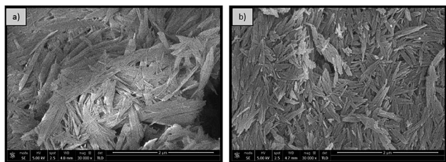
Fig. 4 SEM micrographs of \gamma -Al 2 O 3 nanorods synthesised for 20 hours with 1 M NaOH (0.77 NaOH : Al molar ratio) at (a) 180 °C and (b) 200 °C.
