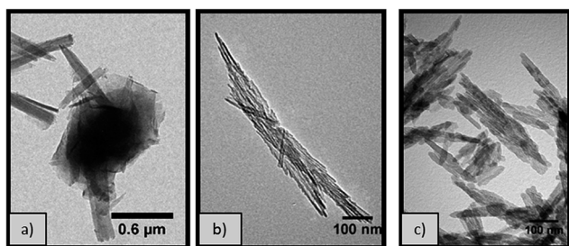
Fig. 3 TEM micrographs of \gamma\text{-Al}_2\text{O}_3 obtained from hydrothermal treatment for 20 hours with 1 M NaOH (0.77 NaOH : Al molar ratio) at (a) 170\text{ }^{\circ}\text{C} (b) 180\text{ }^{\circ}\text{C} and (c) 200\text{ }^{\circ}\text{C} .
