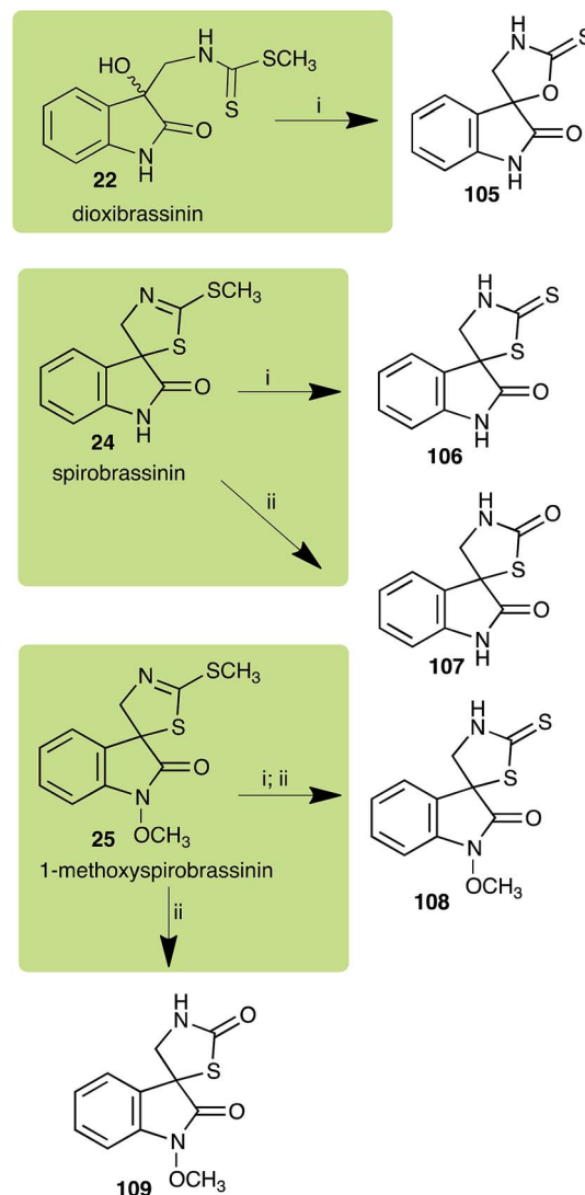
Scheme 7 Detoxification of the cruciferous phytoalexins dioxibassinin ( 22 ), spirobassinin ( 24 ) and 1-methoxyspirobassinin ( 25 ) by plant fungal pathogens: (i) Leptosphaeria maculans (brown mustard virulent isolates); (ii) Sclerotinia sclerotiorum .
