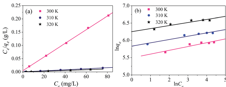
Fig. 14 Adsorption isotherms for the adsorption of mercury(II) onto magnetic PPy-GO: Langmuir (a) and Freundlich (b) models. Conditions: pH = 7 \pm 0.1 , RSL = 0.05 \text{ g L}^{-1} , C_0 = 20\text{--}100 \text{ mg L}^{-1} .
