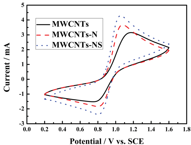
Fig. 3 Cyclic voltammograms of glassy carbon electrodes modified by different MWCNTs samples at the scan rate of 20 \text{ mV s}^{-1} in a 2.0 \text{ mol L}^{-1} \text{ VOSO}_4 + 3.0 \text{ mol L}^{-1} \text{ H}_2\text{SO}_4 electrolyte solution.
