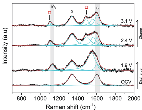
Fig. 12 In situ electrochemical SHINERS spectra of O_2 saturated 0.5 M LiClO_4 /DMSO on a carbon black (SuperC/PTFE) composite electrode. The carbon G-band and position of the LiO_2 band are highlighted in greyscale. Fitted bands are in cyan and the total fitting is in red.
