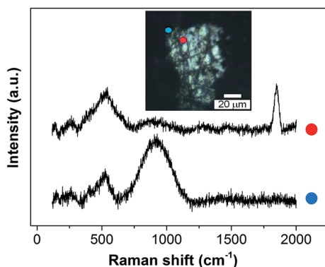
Fig. 9 Ex situ SHINERS spectra collected on lithium metal after cycling in an O 2 saturated 0.25 M LiClO 4 -in-diglyme electrolyte showing the non-homogeneous film formed during discharge.
