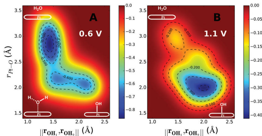
Fig. 3 Two-dimensional free energy contours for water formation through the ER mechanism at 0.6 V potential (A) and 1.1 V potential (B). The free energy barrier for water formation ( \text{H}_3\text{O}^+ + e^- + \text{*OH} \rightarrow \text{H}_2\text{O} + \text{H}_2\text{O} ) derived from the QM RMD simulation is \Delta G^\ddagger = 0.16 eV for 0.6 V and \Delta G^\ddagger = 0.39 eV for 1.1 V. After correcting for the change in the potential along the reaction path (the potential goes up when the e^- is used to form water) to obtain the barrier for constant potential we obtain \Delta G^\ddagger = 0.12 eV for U = 0.6 V and 0.35 eV for U = 1.1 V. The potentials were controlled by adding one \text{H}_3\text{O}^+ ( \text{H}_3\text{O}^+ + e^- ) for the case of 0.6 V and adding one \text{H}_3\text{O}^+ and one Cl ( \text{H}_3\text{O}^+ + \text{Cl}^- ) for the case of 1.1 V. The two collective variables are: (1) norm of r_{\text{OH}_a} and r_{\text{OH}_b} , ( \|r_{\text{OH}_a}, r_{\text{OH}_b}\| = \sqrt{r_{\text{OH}_a}^2 + r_{\text{OH}_b}^2} , where, \text{H}_a is the hydrogen in \text{OH}^* , and \text{H}_b is the nearest hydrogen from the nearby \text{H}_2\text{O} .) It is necessary to constrain two OH distances to ensure that the final product is water ( \text{H}_a\text{--O--H}_b ). When water forms, \|r_{\text{OH}_a}, r_{\text{OH}_b}\| is about 1.41 Å. (2) The distance between O ( \text{OH}^* ) and Pt ( r_{\text{Pt--O}} ).
