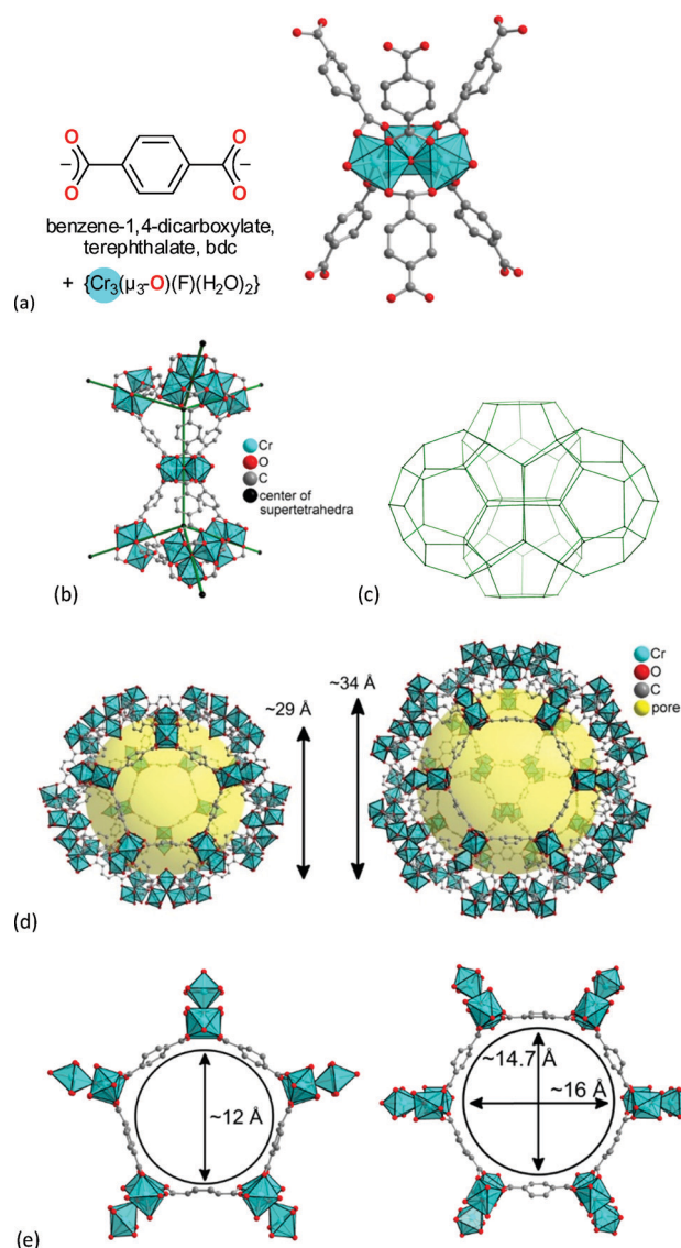
Fig. 8 (a) Ligand and metal building blocks in the trinuclear {Cr 3 (μ 3 -O)(O 2 C-) (F/OH)(H 2 O) 2 } building unit; (b) supertetrahedra; (c) mesoporous zeotypic network; (d) small cage with pentagonal windows and large cage with pentagonal and hexagonal windows; (e) dimensions of pentagonal and hexagonal cage window apertures. Objects in (a) to (e) are not drawn to scale. Graphics have been created from the deposited cif-file for MIL-101Cr (CSD-Refcode OCUNAK). 51
