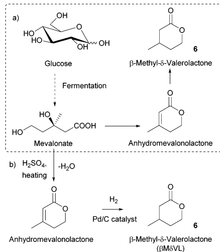
Fig. 5 (a) Biochemical synthesis of \beta M \delta V; (b) semisynthetic production of \beta M \delta V from mevalonate.
