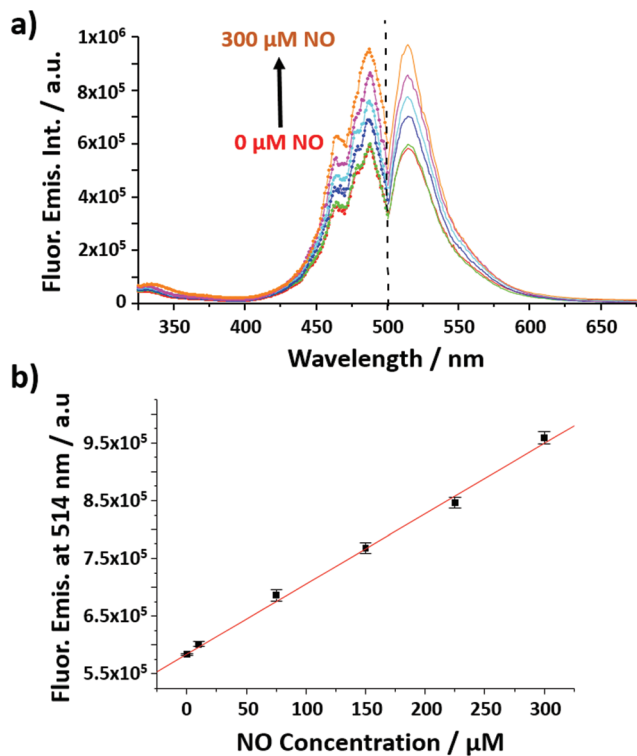
Fig. 2 (a) Fluorescence excitation (left; \lambda_{\text{ems}} = 514 nm) and emission (right; \lambda_{\text{exc}} = 492 nm) spectra of the NO nanobiosensor in the presence of increasing concentrations of NO (from 0 to 300 \mu\text{M} ). (b) Calibration curve of the NO nanobiosensor obtained from the fluorescence emission intensity at 514 nm as a function of the concentrations of NO; error bars show the mean error of 3 replicates. y = 1217x + 584141 .
