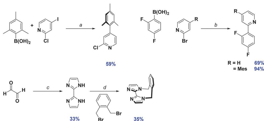
Scheme 1 Synthesis of C a N and N a N ligands. Reagents and conditions: a K 2 CO 3 , 1,4-dioxane/water (2:1 v/v), Pd(PPh 3 ) 4 (5 mol%), 100 °C, 72 h. b Na 2 CO 3 , 1,4-dioxane/water (2:1 v/v), Pd(PPh 3 ) 4 (5 mol%), 100 °C, 19 h. c NH 4 OAc, H 2 O, 40 °C, 8 h. d MeCN, NaOH (35% w/v), 82 °C, 16 h.
