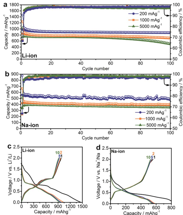
Fig. 2 Electrochemical performance of SnSb NCs. Capacity retention of SnSb NCs in (a) Li-ion and (b) Na-ion half-cells at currents of 200, 1000 and 5000 mA g -1 . Galvanostatic charge and discharge curves of SnSb NCs in (c) Li-ion and (d) Na-ion half-cells at a current of 200 mA g -1 . All measurements were performed in the potential range of 0.005–2.0 V.
