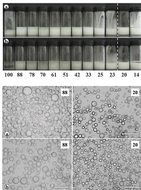
Fig. 4 (upper) Photographs of glass vials containing (a) sunflower oil–50 cS PDMS and (b) olive oil–50 cS PDMS emulsions (both 1 : 1) after 1 month stabilised by 1 wt% of DCDMS-coated fumed silica particles with different % SiOH on their surfaces (given). Emulsions invert from S/V to V/S around dashed line. (lower) Corresponding optical micrographs of the emulsions at selected % SiOH (given). Scale bars = 200 μm.
