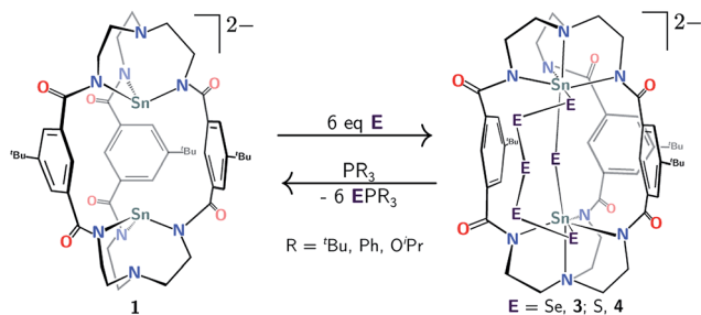
Scheme 2 Reactivity of [Sn_2(mBDCA-5t)]^{2-} ( 1 ) with elemental selenium and sulfur to generate [(\mu-E)_5Sn_2(\mu-E)(mBDCA-5t)]^{2-} ( E = \text{Se, S, 3, 4} ).
