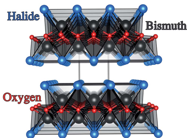
Fig. 1 Crystal structure of the BiOX systems (space group P4/nmm , D_{4h} symmetry) with stoichiometric \text{X–Bi–O–Bi–X} bi-layers stacked along the c axis. Bismuth, oxygen and halide ions are denoted by black, red and blue spheres, respectively.
