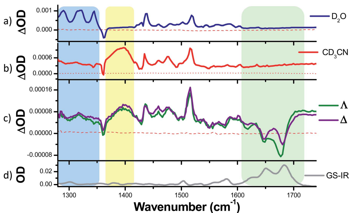
Fig. 8 TRIR spectra recorded 35 ps after 400\text{ nm} excitation of (a) 1\cdot 2\text{Cl}^- ( 500\text{ }\mu\text{M} ) in \text{D}_2\text{O} , (b) 1\cdot 2\text{PF}_6^- ( 500\text{ }\mu\text{M} ) in \text{CD}_3\text{CN} and (c) \Delta - and \Lambda -[ 1 ] 2\text{Cl}^- ( 400\text{ }\mu\text{M} ) and a duplex DNA oligonucleotide \text{d}(\text{TCGGCGCCGA})_2 ( 500\text{ }\mu\text{M} duplex) and (d) FTIR spectrum of oligonucleotide \text{d}(\text{TCGGCGCCGA})_2 ( 500\text{ }\mu\text{M} duplex) in deuterated potassium phosphate buffer ( 50\text{ mM} ) pH 7. The blue and yellow coloured regions highlight the characteristic transient bands for the excited state of 1 , while the green coloured region highlights the bands associated with the DNA base pairs.
