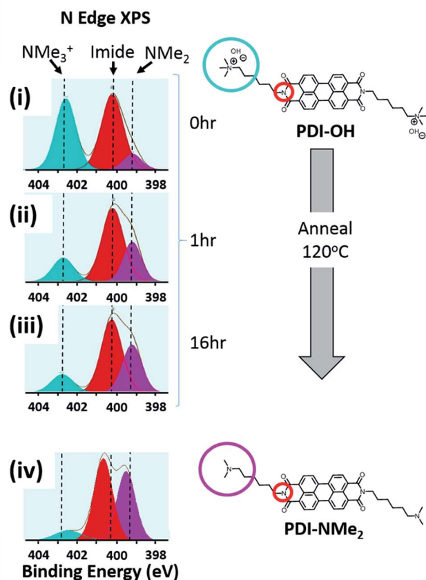
Fig. 2 Conversion of NMe 3 + to NMe 2 in PDI-OH proceeds upon thin film annealing at 120 °C ((i) 0 h, (ii) 1 h, (iii) 16 h) as observed via XPS (N 1s spectra). As expected, after extended annealing, the XPS spectrum of films of PDI-OH closely resembles that of PDI-NMe 2 (iv).
