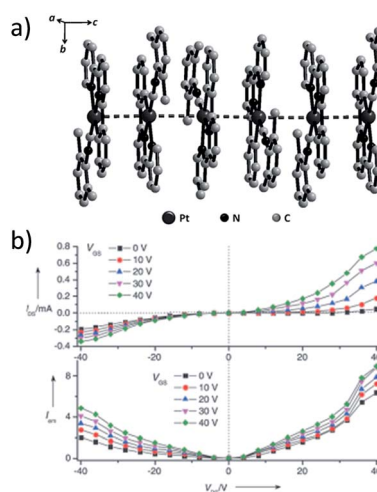
Fig. 9 (a) Crystal packing diagram of 61 ·H 2 O. The PF 6 - and water molecules are omitted for clarity. (b) Output characteristics ( I_{DS} vs. V_{DS} ) and electroluminescence intensity ( I ) of an OLEFET device with nanowires of 61 after annealing at 350 K (adapted with permission from ref. 112. Copyright 2008, Wiley-VCH Verlag GmbH & Co. KGaA).
