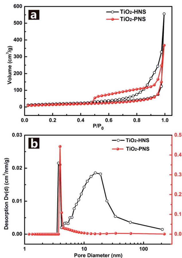
Fig. 3 (a) Nitrogen adsorption/desorption isotherms and (b) Barret–Joyner–Halenda (BJH) pore-size distribution curves of the \text{TiO}_2 -HNSs and \text{TiO}_2 -PNSs.
