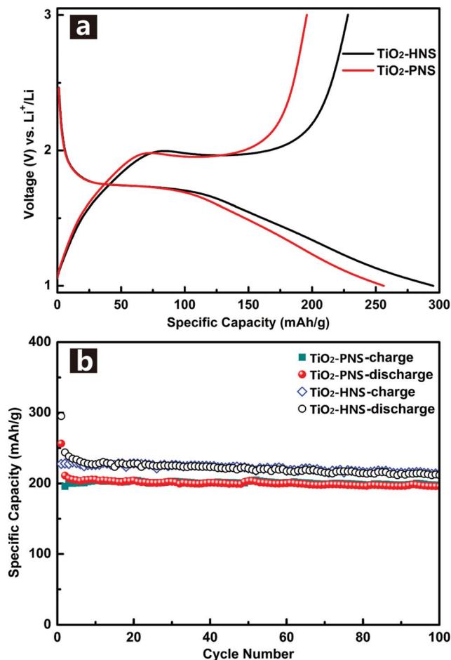
Fig. 5 (a) Initial charge–discharge voltage profiles and (b) cycling performance of the \text{TiO}_2\text{-HNSs} and \text{TiO}_2\text{-PNS} at a current rate of 1 C between 1.0 and 3.0 V.
