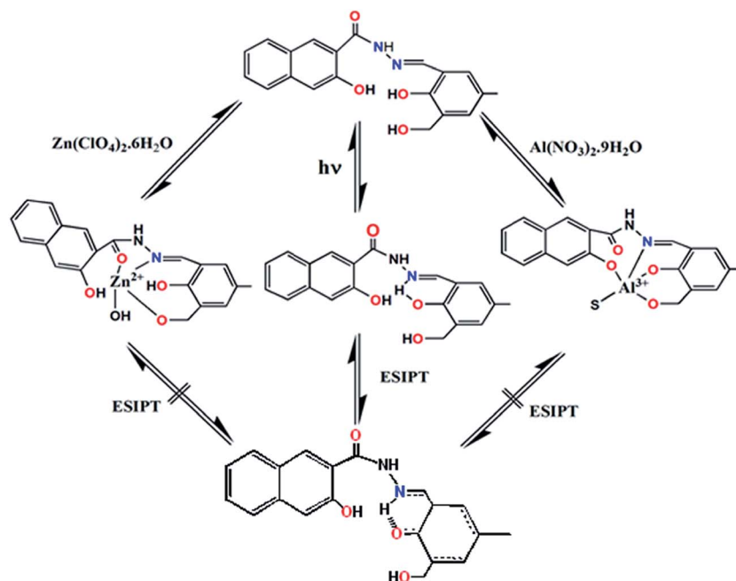
Scheme 1 Proposed ESIPT in the compound \text{H}_3\text{SAL-NH} (1).
