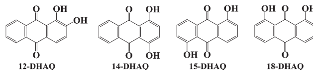
Scheme 1 Chemical structures of the investigated dihydroxyanthraquinone derivatives (12-DHAQ, 14-DHAQ, 15-DHAQ and 18-DHAQ).
