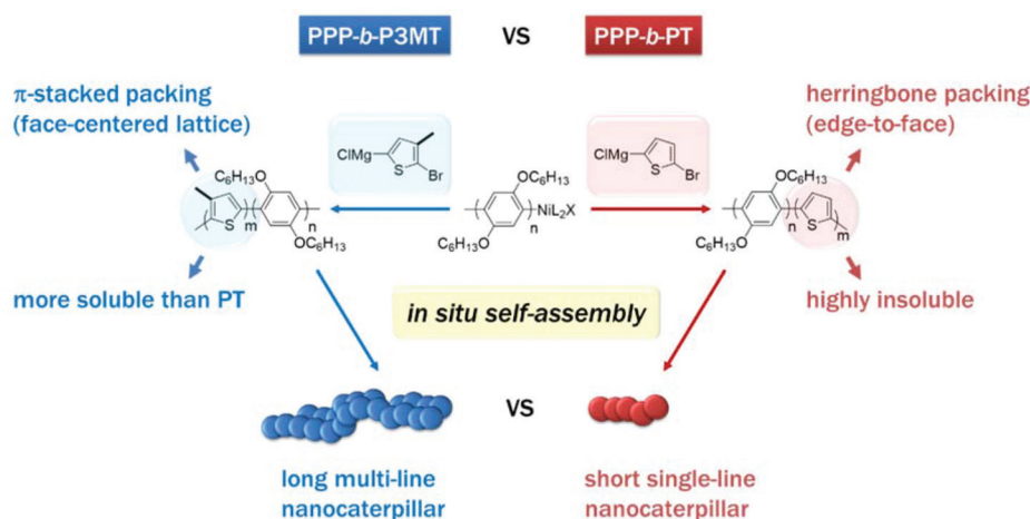
Scheme 1 Comparison between in situ nanoparticulation of PPP- b -P3MT and PPP- b -PT. Note the different solubility and packing modes of P3MT and PT.
