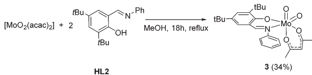
Scheme 3 Synthesis of monosubstituted complex 3 .
