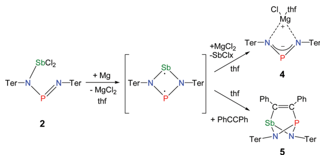
Fig. 8 Reduction of 2 with magnesium and trapping of the transient biradical.
