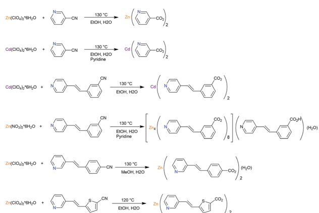
Fig. 14 Synthesis of 2D coordination polymers consisting of d^{10} metals and bridging p -pyridine carboxylate ligands. Adapted from ref. 80.
