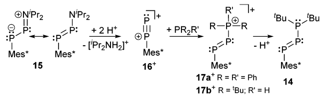
Scheme 6 Protonation of \mathbf{15} in the presence of phosphanes leading to \sigma^2-\sigma^2-\sigma^4 -( \mathbf{17}^+ ) and \sigma^2-\sigma^2-\sigma^4 -compounds ( \mathbf{14} ) formally via \mathbf{16}^+ . Scheme simplified for clarity reason.
