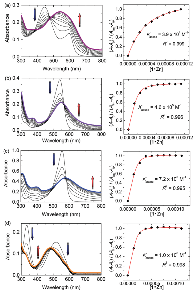
Fig. 2 UV-vis spectra of the diol-dye ( 2.0 \times 10^{-5} M ) upon the addition of 1·Zn in HEPES buffer (10 mM) with sodium chloride (10 mM) at 7.5 at 25 °C. [\mathbf{1·Zn}] = 0-0.11 mM. (a) PV, (b) PR, (c) BPR and (d) ARS.
