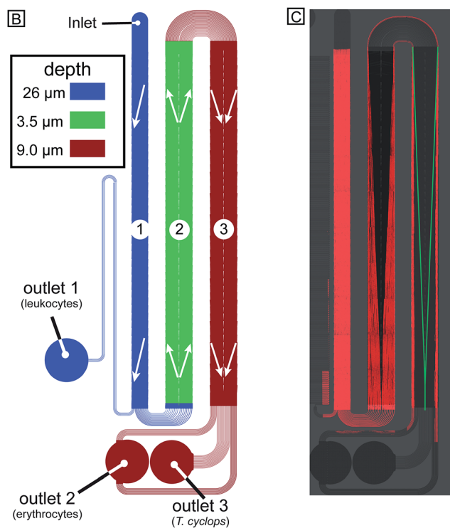
Fig. 3 (A) Basic principle of how orientation changes the effective size of particles of different shape. (B) Schematic overview with the three different sections colour coded. Arrows represent the direction of displacement in each section. (C) False-coloured mosaic image consisting of 34 time-integrated micrographs showing the trajectories of erythrocytes and the parasites through the device.
