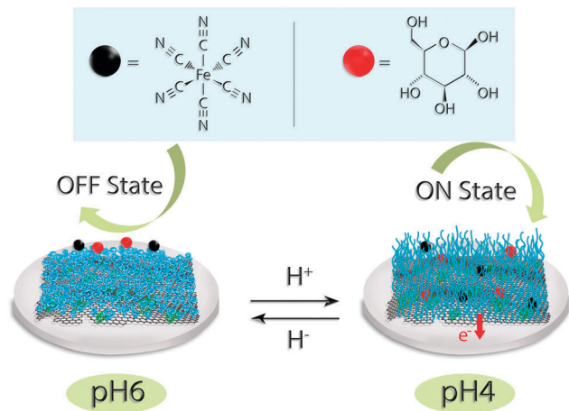
Scheme 1 Schematic representations of a pH-encoded switchable graphene oxide interface at two different states. The tuneable character of the interface was tested using redox-active ferri/ferrocyanide probe (black circle) and glucose as a substrate (red circle). The diffusion of both molecules was controlled by varying the polymer states: at pH 6, (off state) polymer turns to a shrunken state, and at pH 4 (on state), polymer turns to a swelling state.
