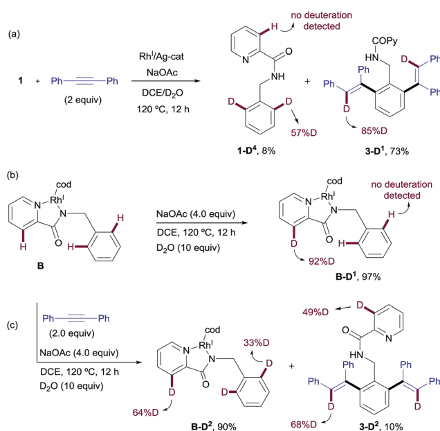
Scheme 11 H/D exchange experiments in the Rh I -promoted C-H functionalization process.
