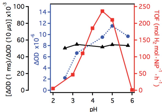
Fig. 4 \text{TOF}_{\text{NiP}(\text{H}_2)} of a homogeneous AA (0.1 M) aqueous solution at different pH values, containing RuP (0.3 μmol, 133 μM) and NiP (0.1 μmol, 44 μM; red squares). Transient absorption signal amplitudes of the NiP bleach at 1 ms (absolute values, blue circles) and transient absorption amplitude ratios of NiP at 1 ms and RuP − at 10 μs (black triangles).
