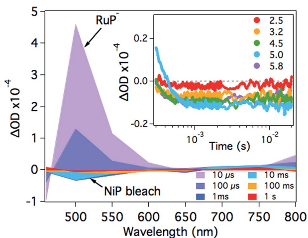
Fig. 3 Transient absorption spectra of a RuP (4 μM) and NiP (8 μM) mixture in the presence of AA (0.1 M) at pH 4.5 as a function of time delay. The inset shows the time profile of the negative signal monitored at \lambda = 500 nm, assigned to the loss of ground state absorption of NiP in the pH range studied. The samples were excited at \lambda = 355 nm.
