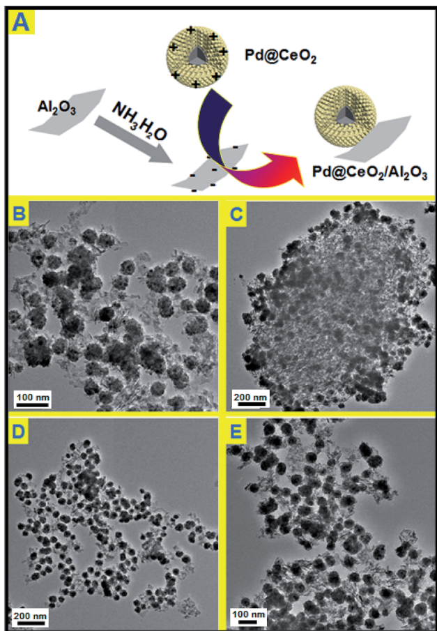
Fig. 4 (A) Schematic representation of the self-assembly of Pd@CeO 2 and commercial γ-Al 2 O 3 ; (B) TEM images of 11 nm-Pd@CeO 2 /Al 2 O 3 ; (C) 13 nm-Pd@CeO 2 /Al 2 O 3 ; (D) 17 nm-Pd@CeO 2 /Al 2 O 3 ; (E) 8 nm-Pd@CeO 2 /Al 2 O 3 .
