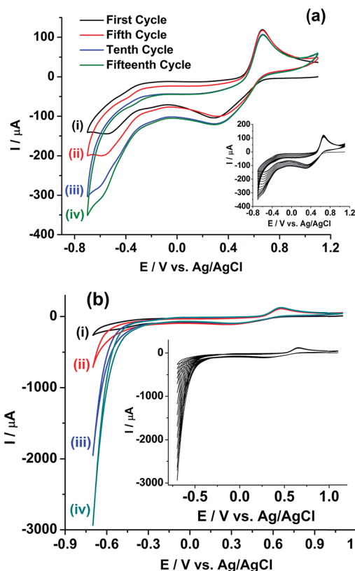
Fig. 7 Cyclic voltammograms of (U, Pu)C FBTR fuel sample on (a) rGO/GC and (b) GC electrodes at a scan rate of 50 \text{ mV s}^{-1} for (i) first, (ii) fifth, (iii) tenth and (iv) fifteenth cycle. The insets show the continuous cyclic voltammograms of 15 cycles.
