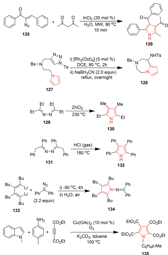
Scheme 19 Substituted pyrrole molecules.
