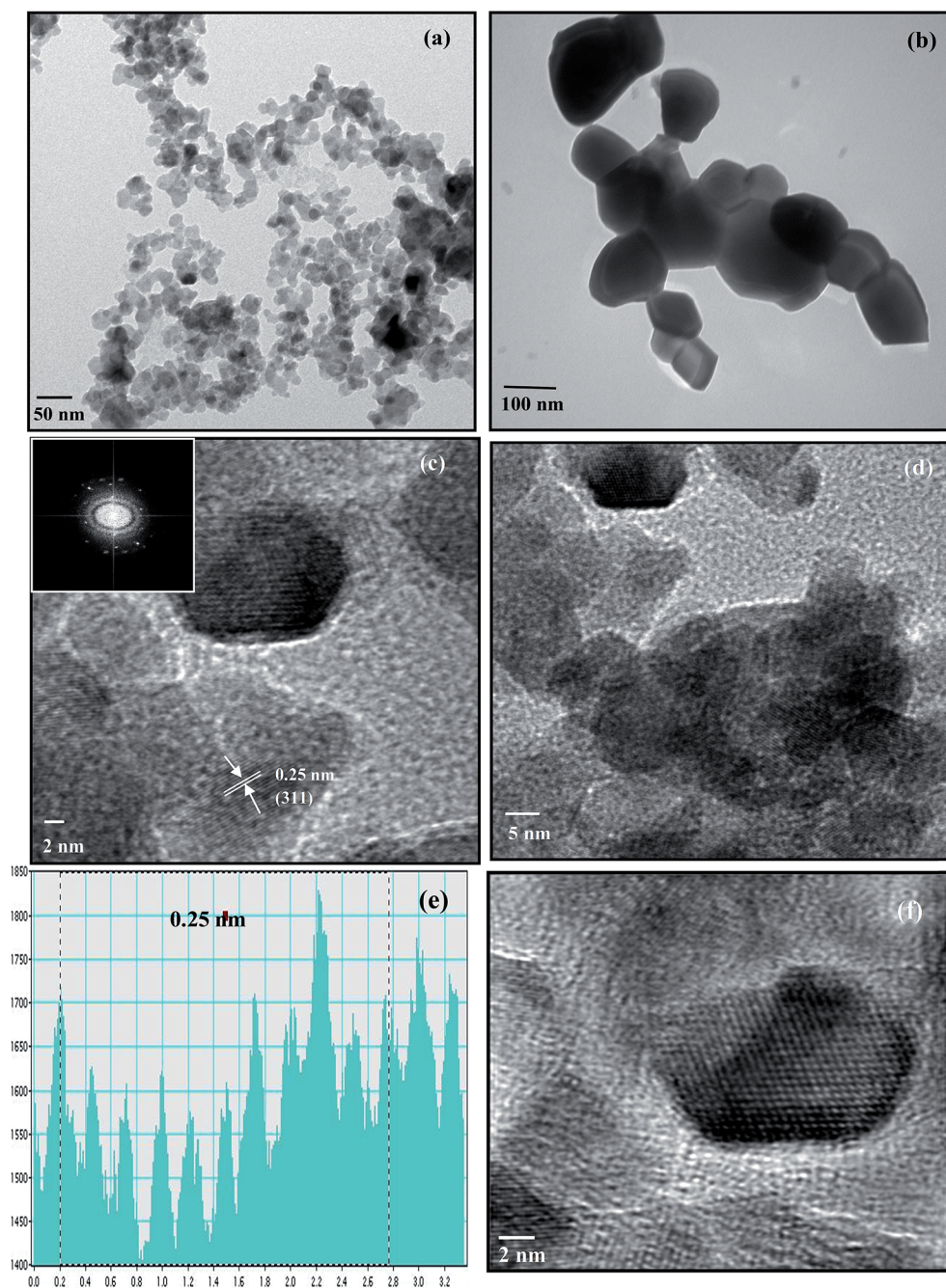
Fig. 1 TEM images of \text{CuFe}_2\text{O}_4 annealed at (a) 400\text{ }^\circ\text{C} and (b) 1000\text{ }^\circ\text{C} , HRTEM images of the \text{CuFe}_2\text{O}_4 nanoparticles at (c) magnification of 2\text{ nm} (inset shows the FFT of \text{CuFe}_2\text{O}_4 ) and (d) magnification of 5\text{ nm} . (e) Frame profile for the average fringe width. (f) Reconstructed image after filtering the FFT pattern from HRTEM.
