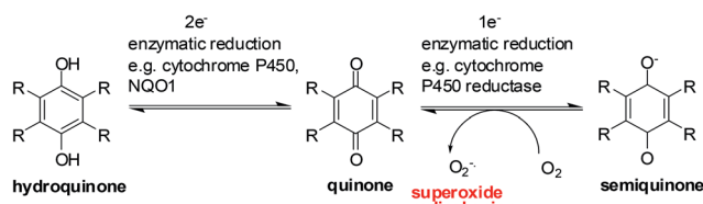
Fig. 6 A general scheme for quinone reduction.
