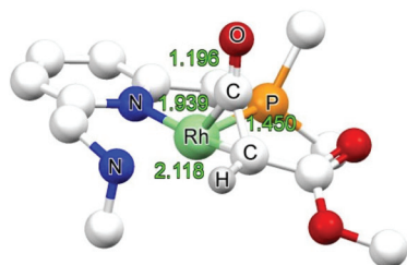
Fig. 3 DFT optimized structure of \text{NHINT3} (bond lengths in Å).
