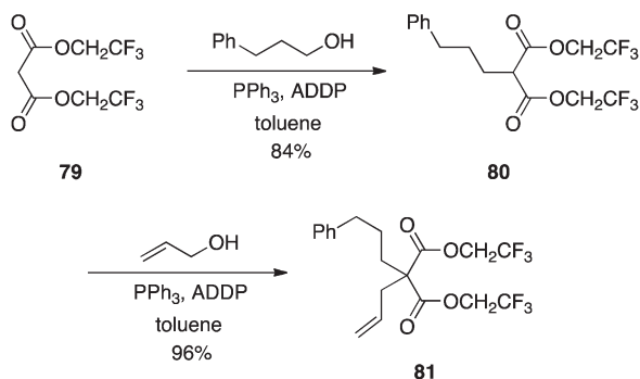
Scheme 25 Activation of the malonate methylene function with greater electron-withdrawing 2,2,2-trifluoroethyl groups allows C-alkylation to proceed smoothly.
