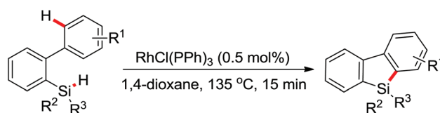
Scheme 374 Rhodium-catalyzed synthesis of silafluorene derivatives.
