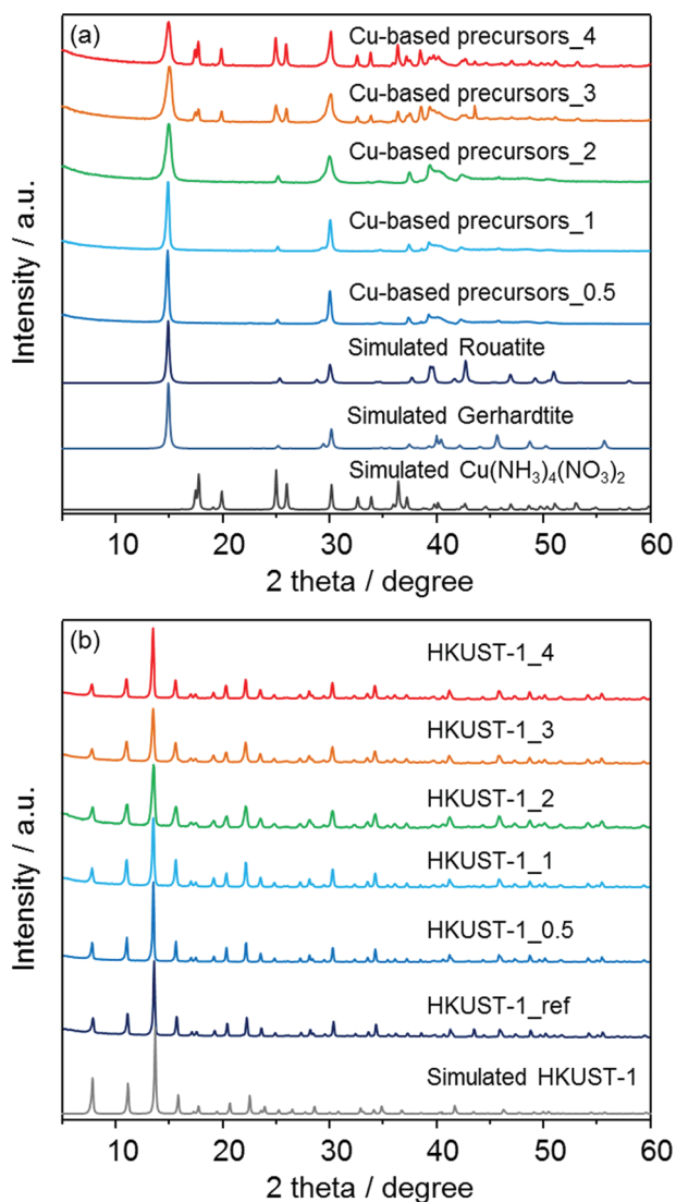
Fig. 3 XRD patterns of (a) the solvent insoluble Cu-based precursors (Cu-based precursors X ) with simulated patterns for Cu 2 (OH) 3 NO 3 (rouatite and gerhardtite) and Cu(NH 3 ) 4 (NO 3 ) 2 and (b) corresponding HKUST-1 X with HKUST-1 ref and simulated pattern for HKUST-1.
