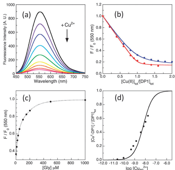
Fig. 4 Determination of apparent K_D' for Cu II -DP1 by direct metal ion titration (a, b) and conditional K_D by ligand competition (c, d) in MOPS buffer (5.0 mM unless otherwise indicated, pH 7.4): (a) quenching of fluorescence emission intensity ( \lambda_{\max} = 550 nm) of apo-DP1 (2.0 μM) upon titration with Cu aq 2+ solution (80 μM); (b) change in F/F_0 for DP1 as a function of [Cu(II)]_{tot}/[DP1]_{tot} concentration: 2.0 μM (red) and 0.2 μM (blue in 0.5 mM buffer). The solid traces are fitting curves of the experimental data to eqn (4), providing apparent \log K_D' = -8.0 \pm 0.1 ; (c) recovery of F/F_0 for Cu II 0.8 -DP1 (2.0 μM) with increasing concentration of competing ligand Gly; (d) curve fitting of [Cu^{II}-DP1]/[DP1]_{tot} versus \log [Cu_{aq}^{2+}] to eqn (8), providing conditional \log K_D = -8.1 \pm 0.2 for Cu II -DP1.
