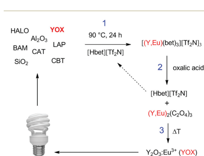
Fig. 13 Overview of the proposed recycling process for lamp phosphor waste, based on the selective dissolution and revalorization of YOX with the protonated functionalized ionic liquid [Hbet][Tf_2N] . Step 1: selective dissolution of YOX, step 2: stripping with pure oxalic acid (regenerates the ionic liquid), step 3: direct resynthesis of YOX.
