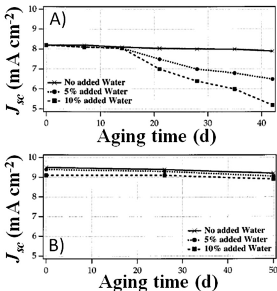
Fig. 17 Long-term stability ( P_{in} = 0.015 \text{ mW cm}^{-2} ) of DSSCs assembled with RTIL-based electrolytes ( I_2 10 mM in HMIL) encompassing different H 2 O contents. Dyes: (A) N3; (B) [Ru(H 2 dcbpy)(mhdcbpy)(NCS) 2 ]. Adapted and reprinted from ref. 231.
