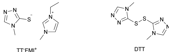
Fig. 13 Structures of the \text{TT}^-\text{EMI}^+/\text{DTT} -based redox couple. Adapted and reprinted from ref. 193.
