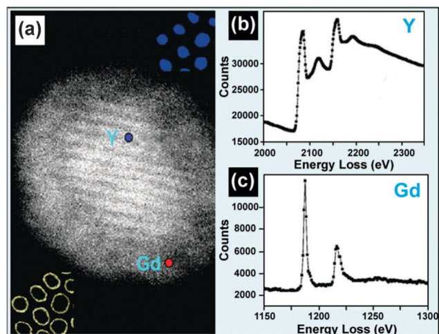
Fig. 12 EELS technique for composition characterization of UC nanocrystals. (a) HADDF image of a single \text{NaYF}_4\text{:Yb/Er} (20/2 mol%) @ \text{NaGdF}_4 core-shell nanocrystal. (b and c) EELS spectra of yttrium \text{L}_{2,3} and gadolinium \text{M}_{4,5} edges obtained from the \text{NaYF}_4\text{:Yb/Er} (20/2 mol%) core and \text{NaGdF}_4 shell as labeled in a. (Reprinted with permission from ref. 134. Copyright 2012, American Chemical Society.)
